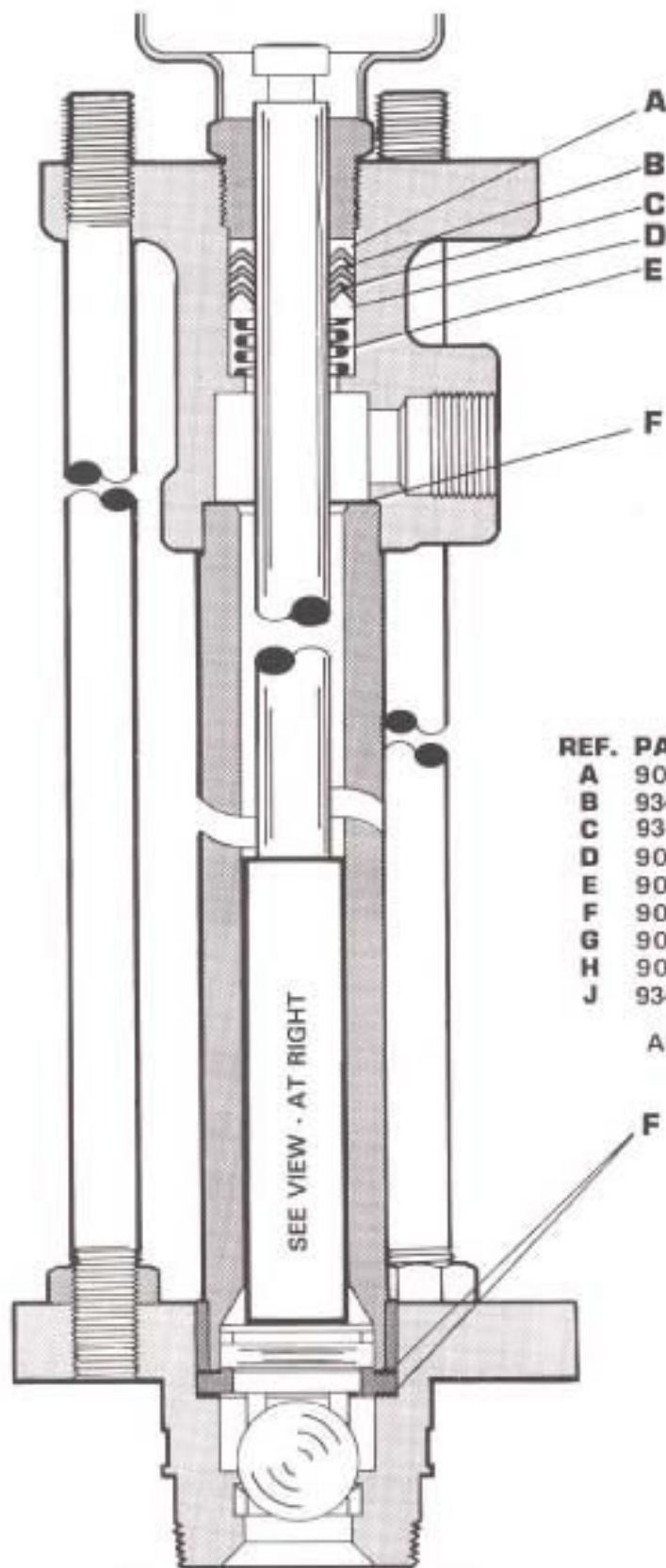
61795 LOWER PUMP END
